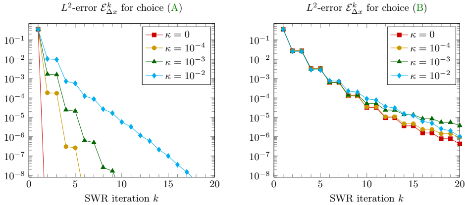
FIGURE 6.7. The L^2 -errors \mathcal{E}_{\Delta x}^k for \lambda = 2 and step-size \Delta x = 0.025 . Left: For the choice (A), the rate of decay of \mathcal{E}_{\Delta x}^k over the number of SWR iterations depends on total mobility \kappa strongly improving when \kappa decreases. Right: For the choice (B), the rate of decay does not improve to finite-step convergence in the hyperbolic limit when \kappa \rightarrow 0 .
