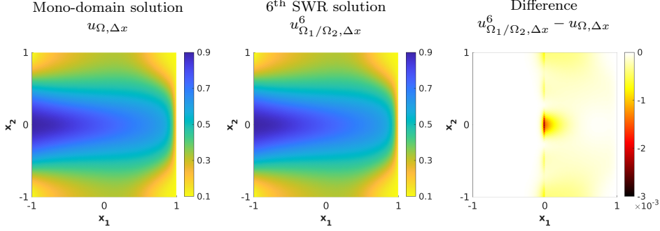
FIGURE 6.8. The numerical mono-domain solution (left) and the SWR solution at the 6 th iteration (middle) are hardly distinguishable from each other for the two-phase equation with Brooks-Corey parameterization at t = 1 using \Delta x = 0.025 . Differences can be observed mostly at the interface \Gamma but less for the wave-front position (right).
