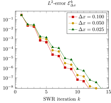
FIGURE 6.9. The L^2 -error \mathcal{E}_{\Delta x}^k decreases monotonically over the number of SWR iterations for the different spatial resolutions for the two-phase equation with Brooks-Corey parameterization with \lambda = 2.5 .
